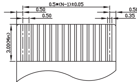
FPC/FFC RECOMMENDED DIM. (THICKNESS: 0.3±0.03)
