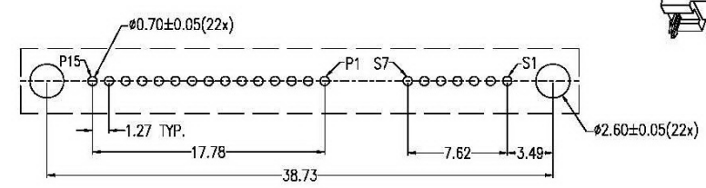
PCB LAYOUT COMPONENT SIDE
