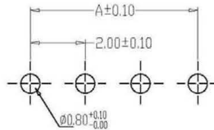
PCB LAYOUT
