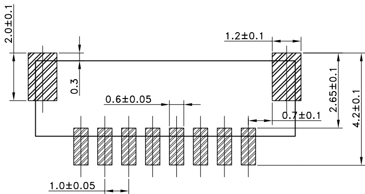
RECOMMENDED P.C. BOARD PATTERN DIM.
