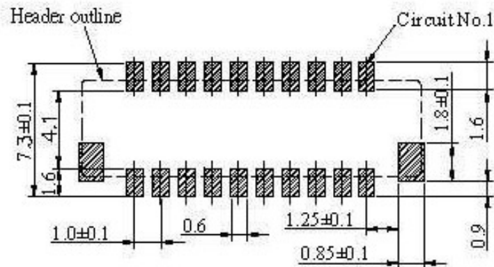
RECOMMENDED P.C. BOARD PATTERN DIM.
