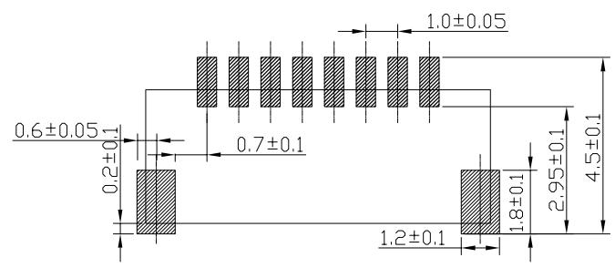
RECOMMENDED P.C.BOARD HOLE DIMM.
