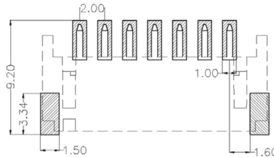
Recommended P.C.B Layout(Top Side)
